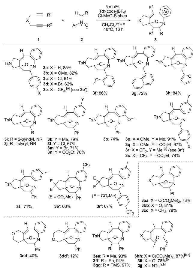
Scheme 2. Substrate scope. Reaction conditions: 1 (0.25 mmol), 2 (0.75 mmol), [Rh(cod)_2]BF_4 (5 mol %), Cl-MeO-Biphep (5 mol %), CH_2Cl_2 (1 mL), THF (1 mL), 40 °C, 16 h; yields of isolated products are reported. [a] The conversion to products 3e , 3r , and 3jj was good, however, they were not isolated because their polarity was similar to that of the corresponding nitron. [b] Reaction conditions: [Rh(cod)_2]BF_4 (5 mol %), Segphos (5 mol %), CH_2Cl_2 (2 mL), 40 °C, 16 h. [c] Yield determined by HPLC.
