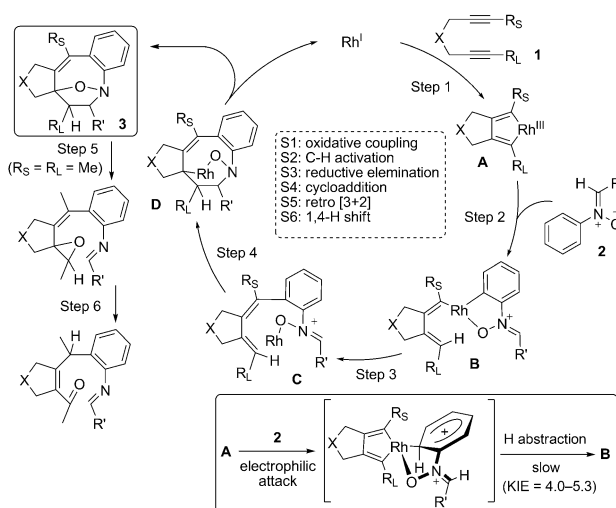
Scheme 3. Proposed mechanism.
